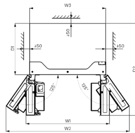
Installation dimensions(mm)
