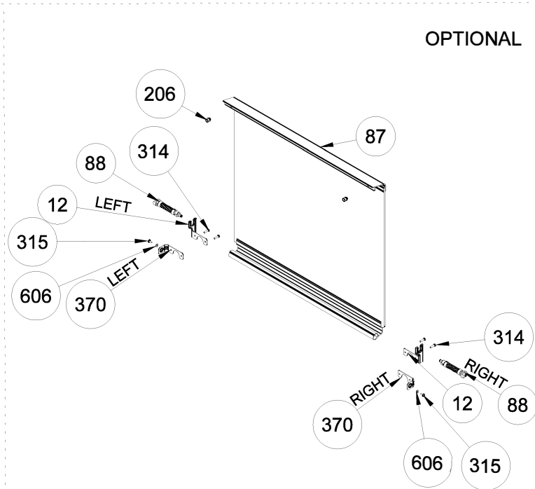
GLASS LID ASSEMBLY POS. NUMBER: 87
