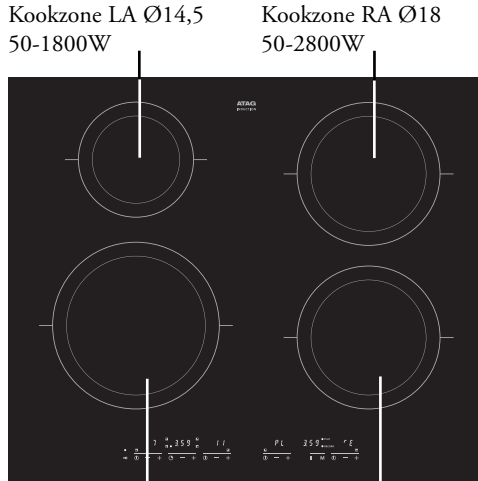
Kookzone LV Ø21 50-3200W
