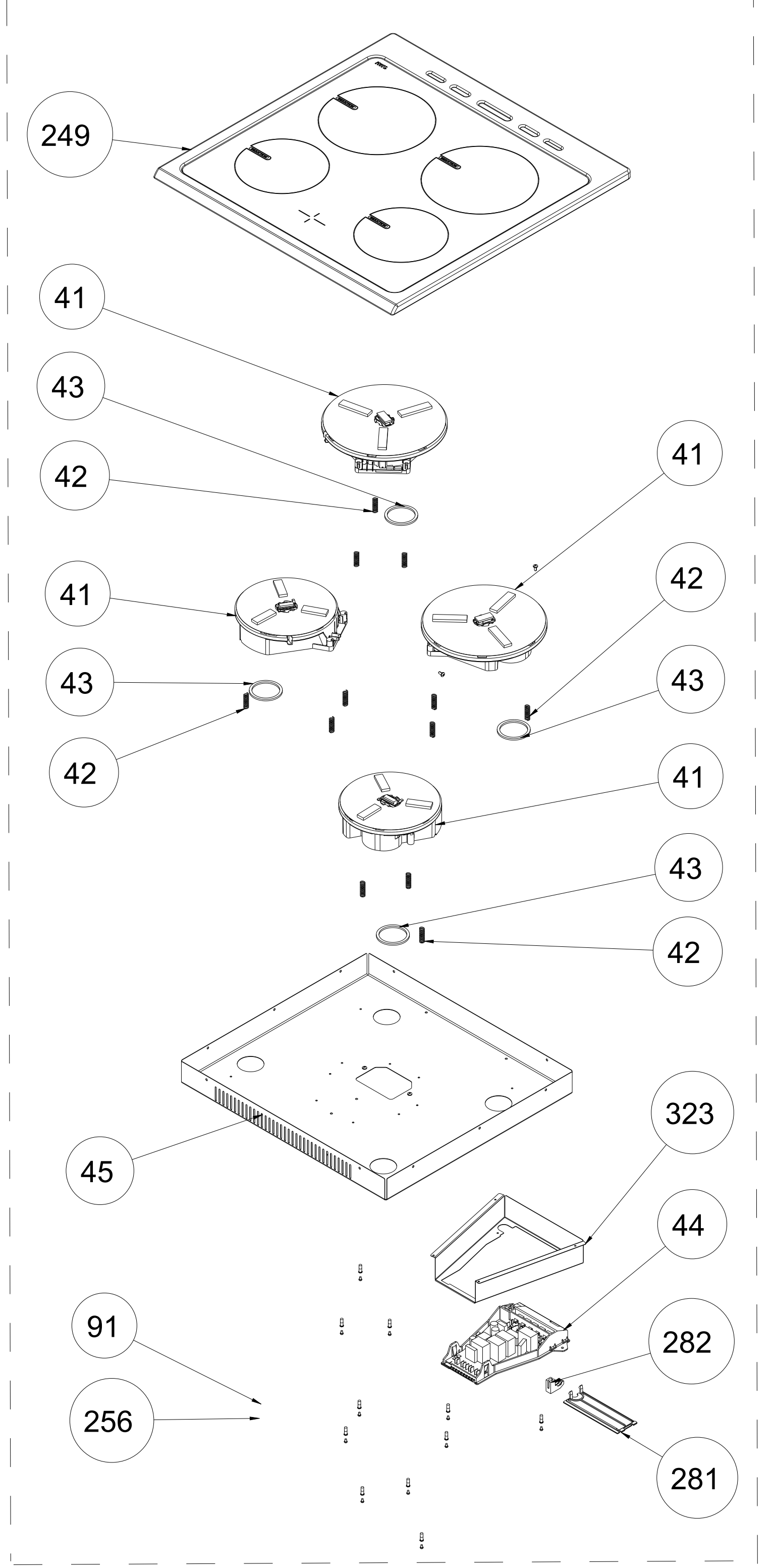
KNOB CONTROL COOKTOP ASSEMBLY
