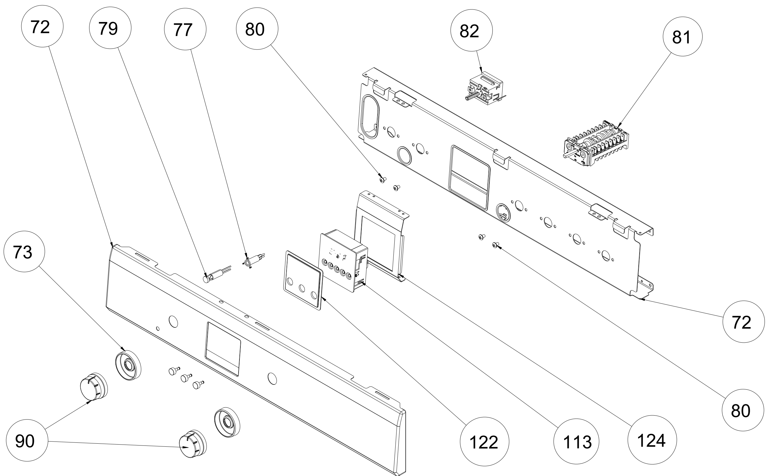
TOUCH CONTROL PANEL ASSEMBLY
