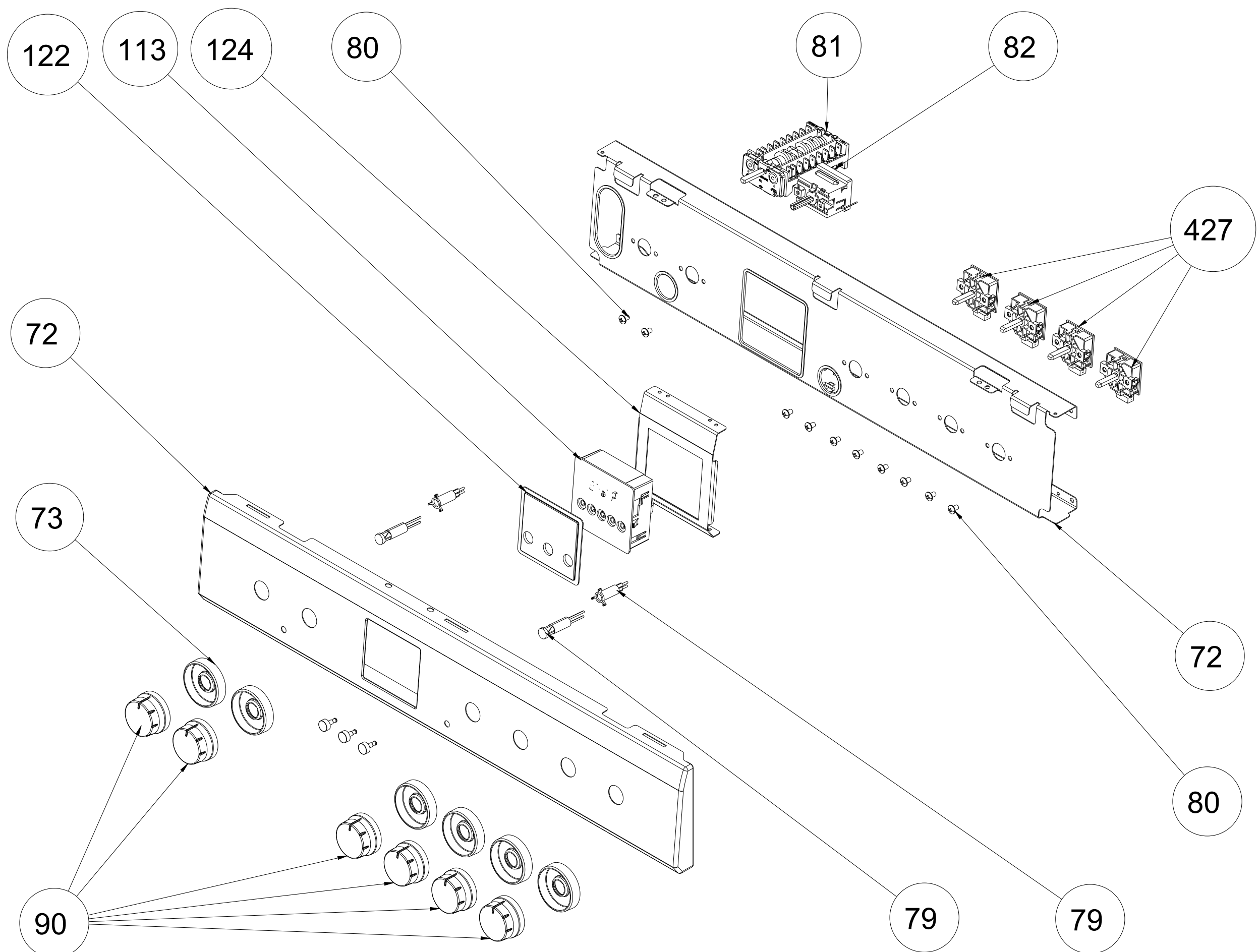
KNOB CONTROL PANEL ASSEMBLY
