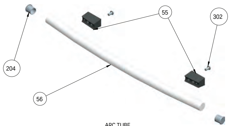
ARC TUBE
