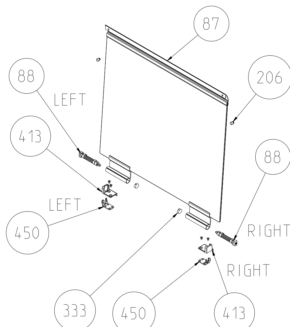
GLASS LID WITH SHORT PROFILE (OPTIONAL)
