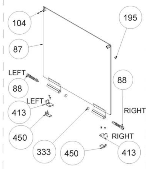
GLASS LID WITH BUMPER OPTIONAL
