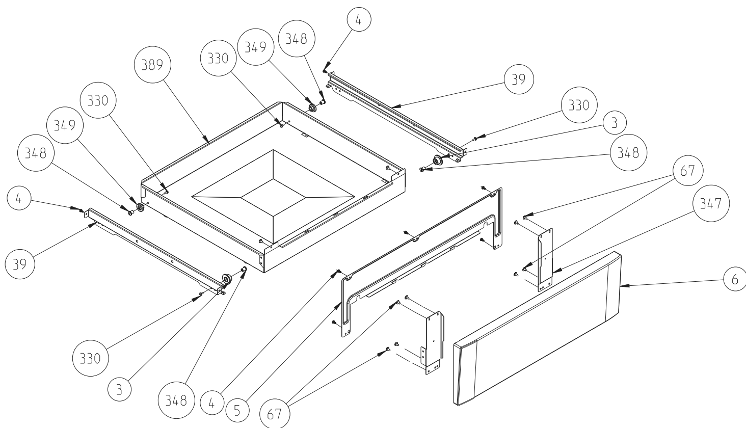
4WG DRAWER ASSEMBLY (OPTIONAL)
