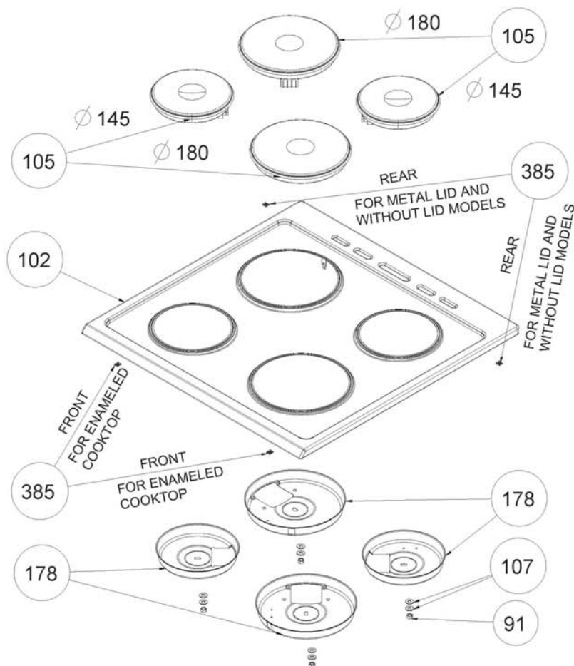
EXPLODED VIEW - COOKTOP ASSEMBLY
