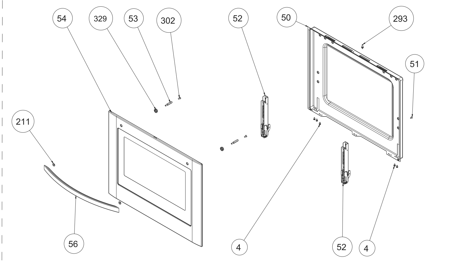
SOLID TYPE - POSITION NO 395 (OPTIONAL)
