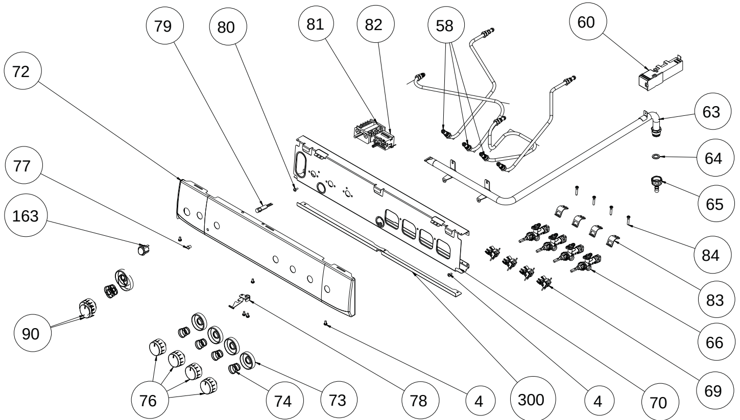
3D- 4GAS - NO TIMER CONTROL PANEL ASSEMBLY
