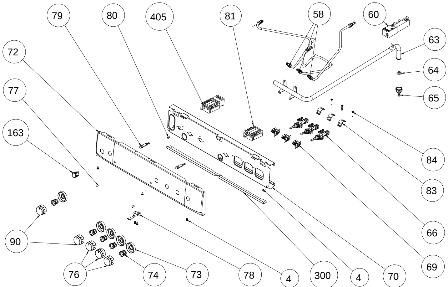
3D- 3GAS+1ELECTRIC - NO TIMER CONTROL PANEL ASSEMBLY
