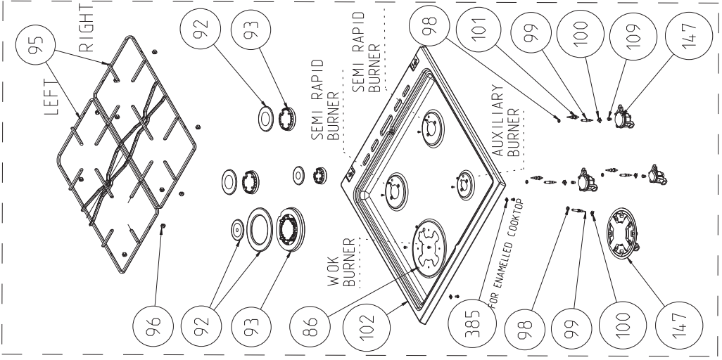
3 GAS+ 1 WOK BURNER
