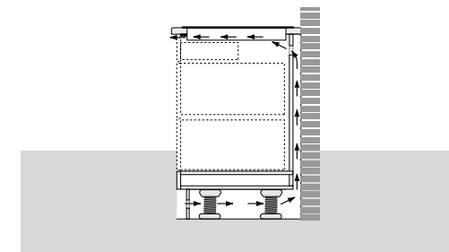
Air circulation under the induction hob.
